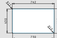
Flushmount installation
