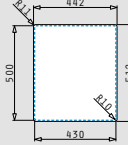
Flushmount installation
