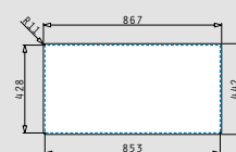
Flushmount installation
